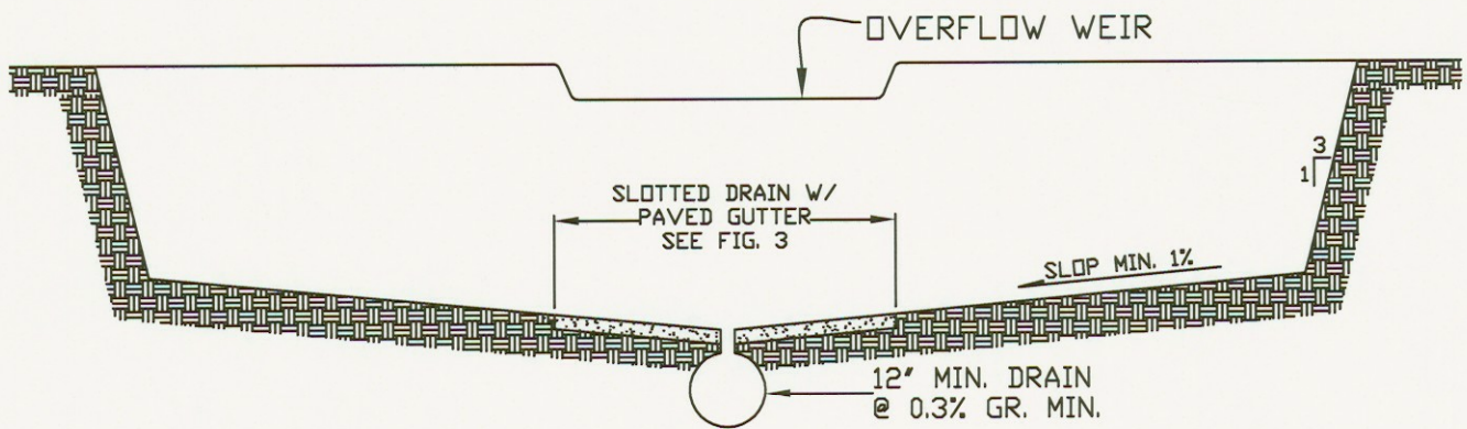
TYPICAL SECTION A-A
