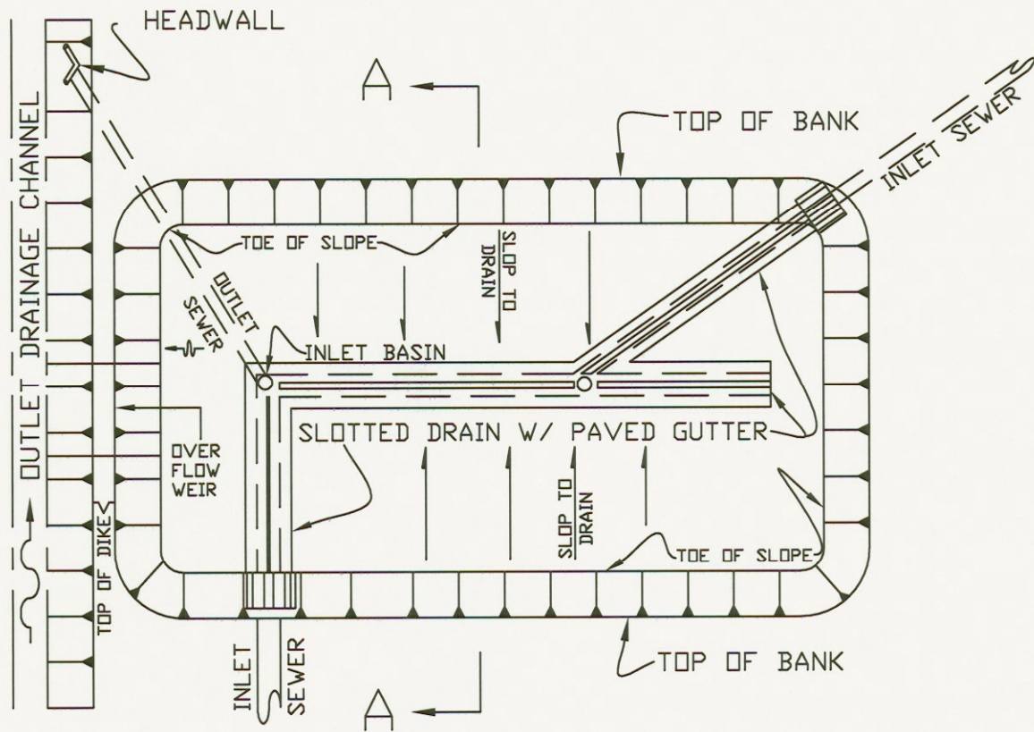
PLAN VIEW RECOMMENDED RETENTION BASIN CONSTRUCTION
